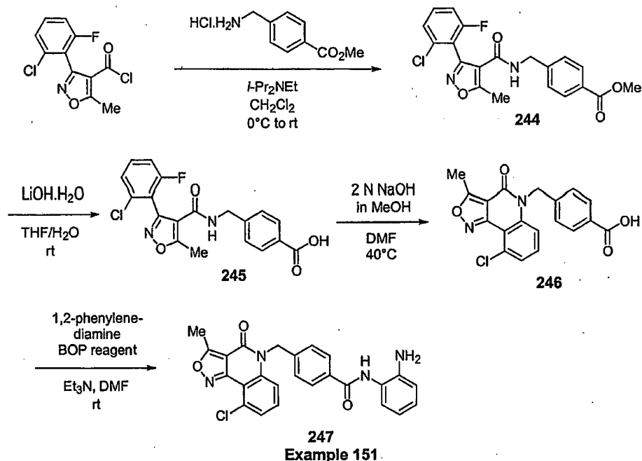
Scheme 40
